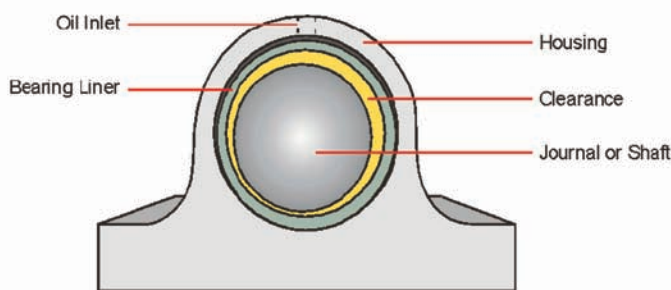
Figure 1 | Pillow-block style journal bearing [Courtesy of Trico Corp.]
