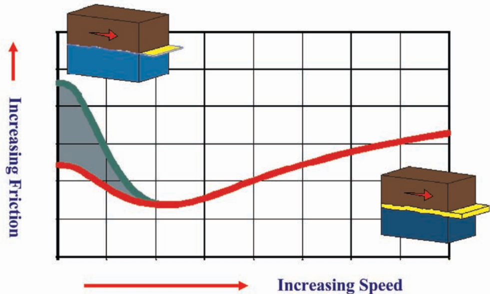
Figure 3 | The Stribeck Curve (Courtesy of Lubcon Consult GMBH)
