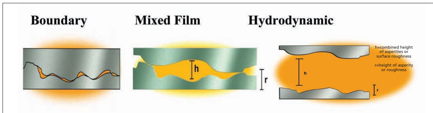
Figure 4 | States of machine surface separation based on change in film thickness
