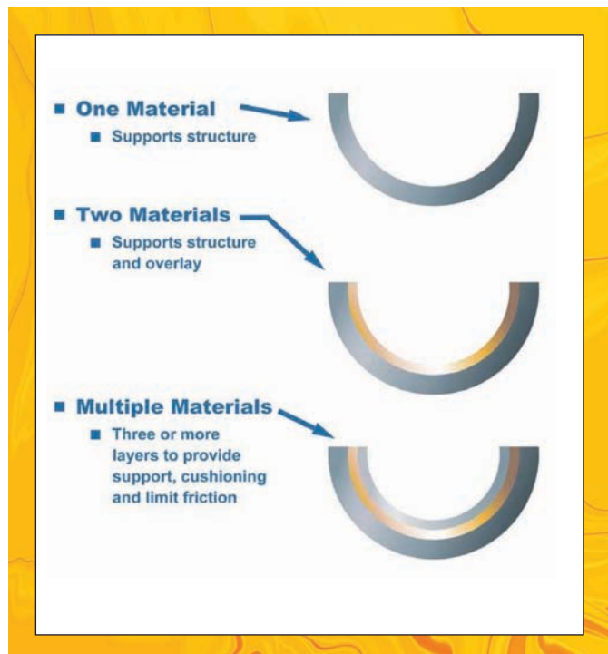
Figure 2 | Journal bearing construction [Courtesy of Trico Corp.]
